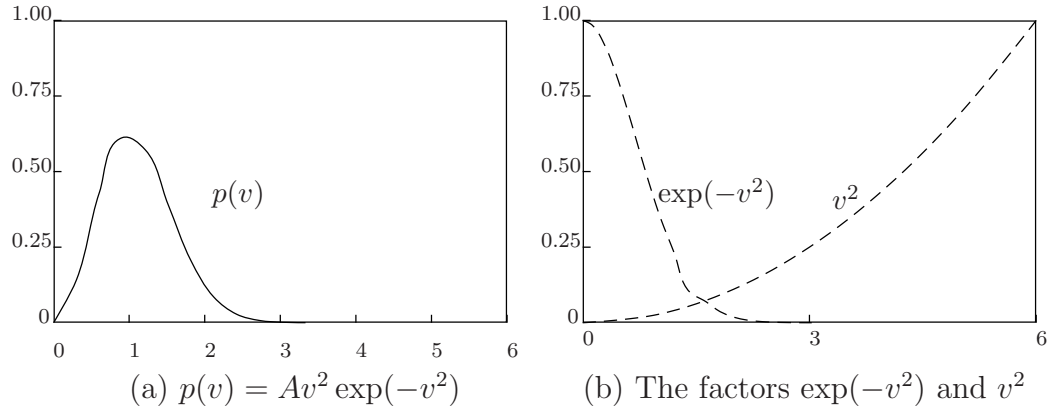
Figure 18. The Maxwell distribution p(v)
